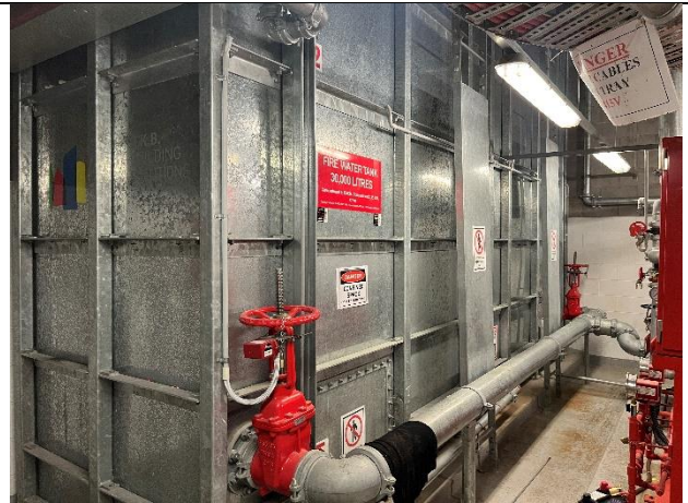
Photo 02. L3, Fire Pump Room, fire water tank.
