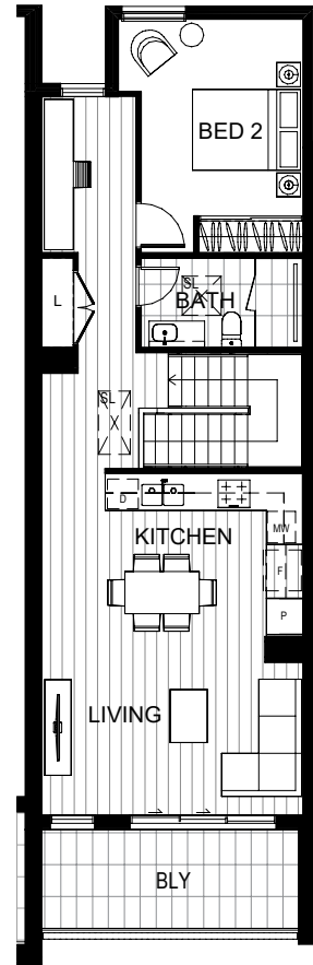
First floor
