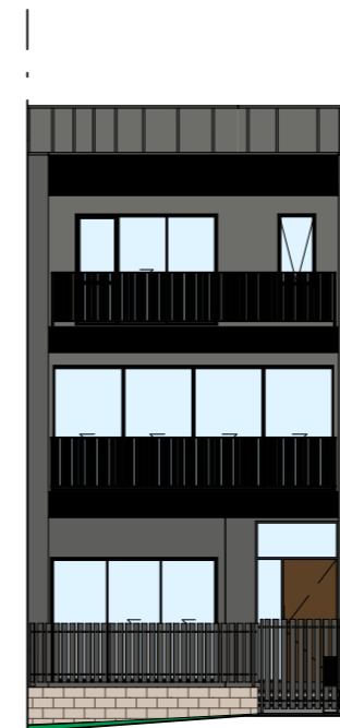
Front Elevation
