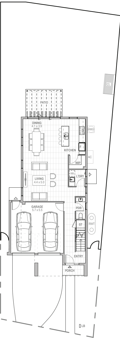
Ground Floor
