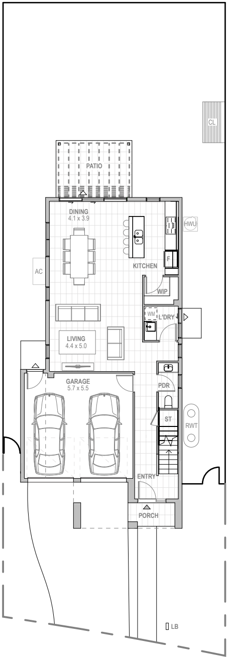
Ground Floor
